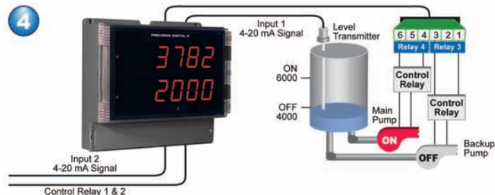
At 4000 gallons, relay 3 turns off and the system returns to normal pump alternation control.
