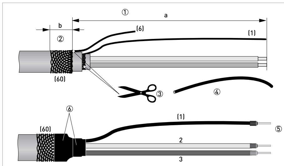
Figure 4-6: Preparing signal cable A, connection to measuring sensor and converter
