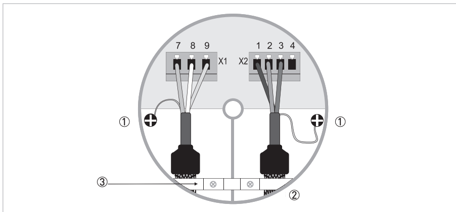
Figure 4-7: Cable connection at sensor and converter side, DS300 cable A
