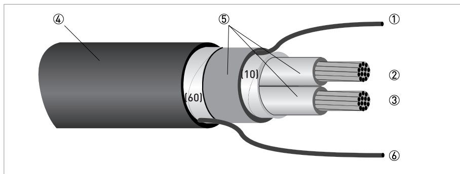
Figure 4-5: Construction of signal cable A
