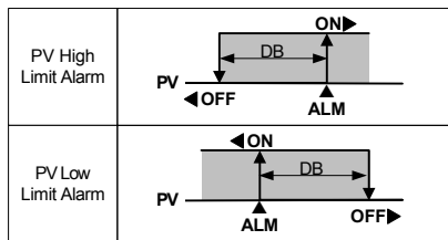
Fig 3: Alarm Operation
